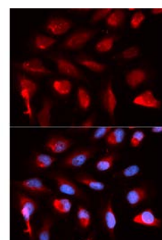
Fig. 2. Immunofluorescence analysis of U2OS cells using PPAR \delta antibody. Blue: DAPI for nuclear staining.
