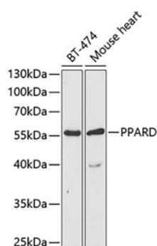
Fig. 1. Western blot analysis of extracts of various cell lines, using PPAR \delta antibody at 1:1000 dilution. Secondary antibody: HRP-labeled Goat Anti-Rabbit IgG(H+L) (A0208) at 1:1000 dilution. Lysates/proteins: 25 \mu g per lane. Blocking buffer: QuickBlock TM Blocking Buffer (P0231). Detection: BeyoECL Star (P0018A). Exposure time:1s.
